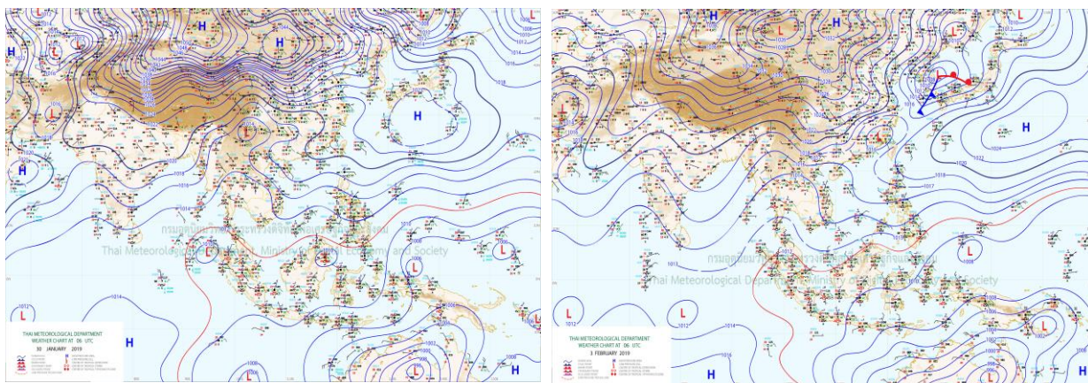
Figure 1: Summary of weather condition over the LMB from 30 Jan and 03 Feb 2020
